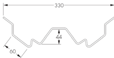
DVA – shallow dry fix valley
