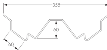
DVB – deep dry fix valley
